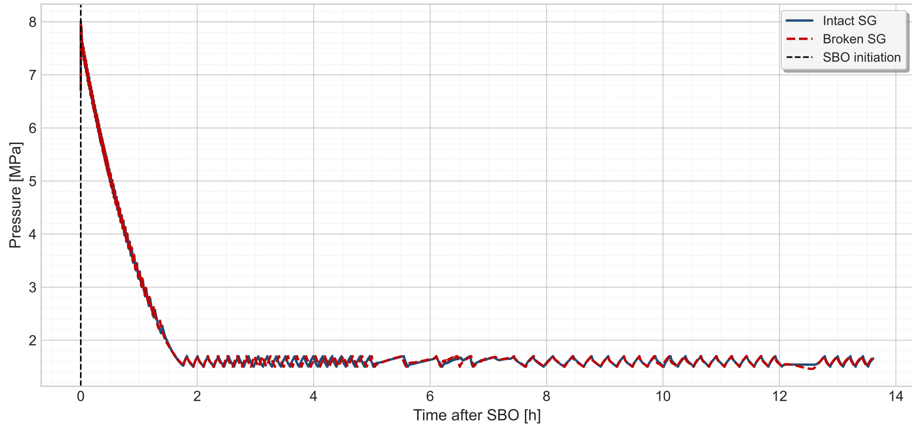
Base Case - Secondary Pressure (SG Cooldown)
